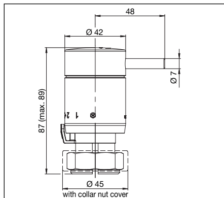
Illustr. 4.1 Dimensions
