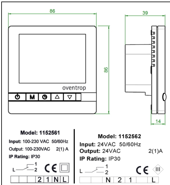
Illustr. 4.1 Dimensions
