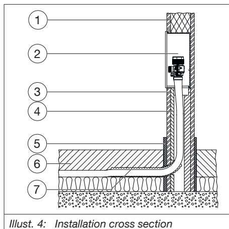
Illust. 4: Installation cross section
