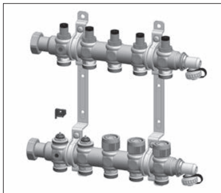
Illustr. 1.1 Stainless steel distributor/collector "Multidis SFQ"
