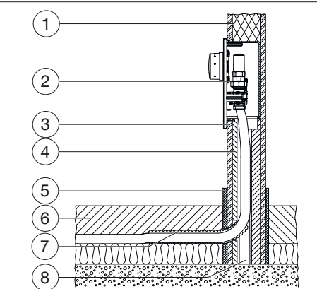
Illust. 7: Installation cross section
