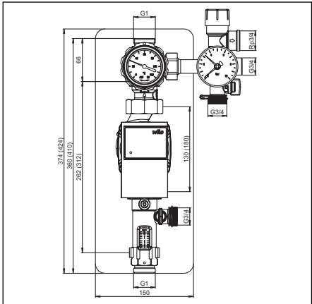
Illustr. 4.1 Pump circuit "Regusol PH-130 (180)" DN25 16
